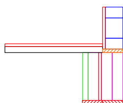
Section A-A. Plinth sat on top of the fillets.
