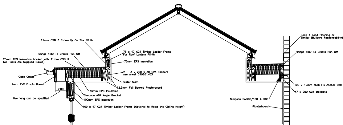
Typical Section Through Roof From Front to Back Sat on Frames
