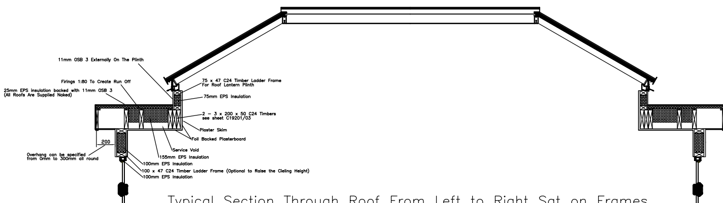
Typical Section Through Roof From Left to Right Sat on Frames
